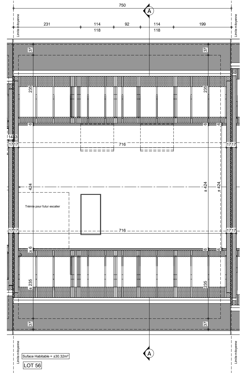
COMBLE AMENAGABLE
